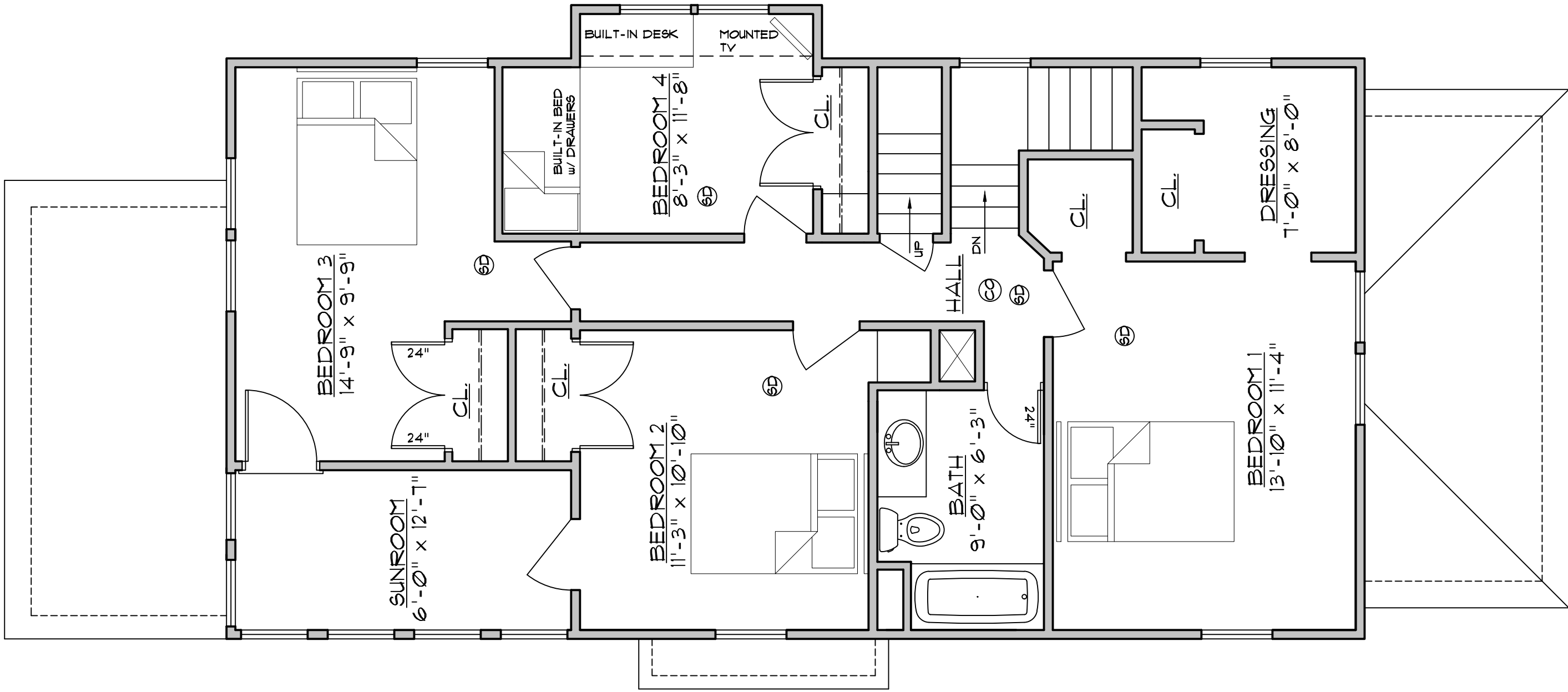
MARKETING SECOND FLOOR PLAN 1/4" = 1'-0"
