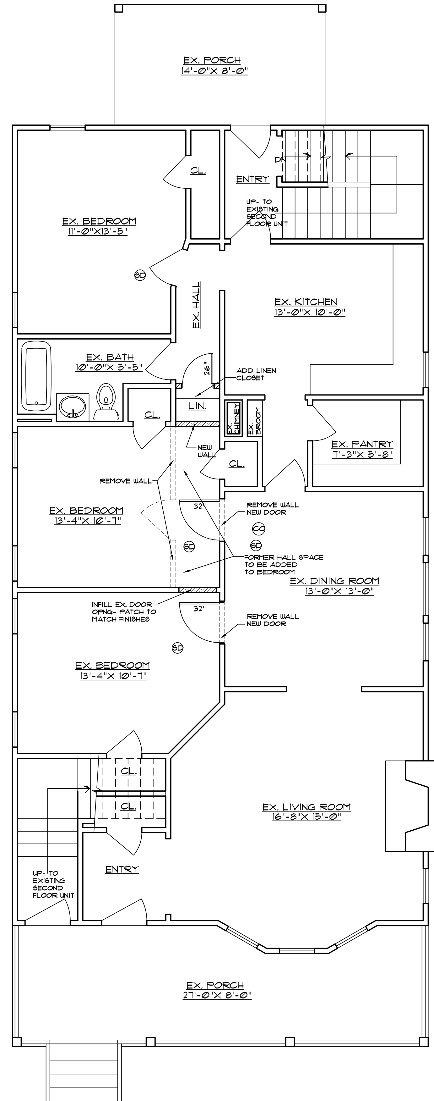
FIRST FLOOR PLAN 1/4" = 1'-0"
