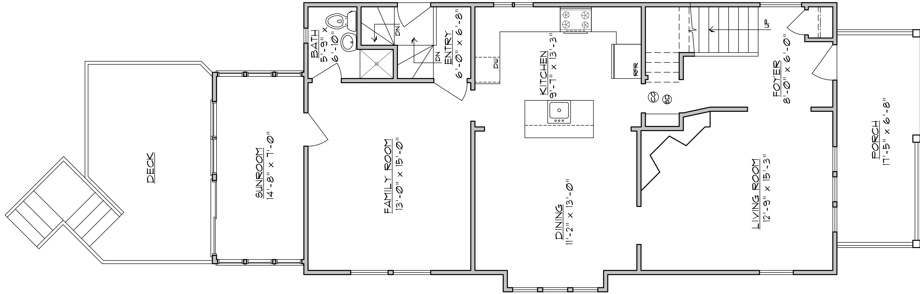
MARKETING FIRST FLOOR PLAN 1/4" = 1'-0"
